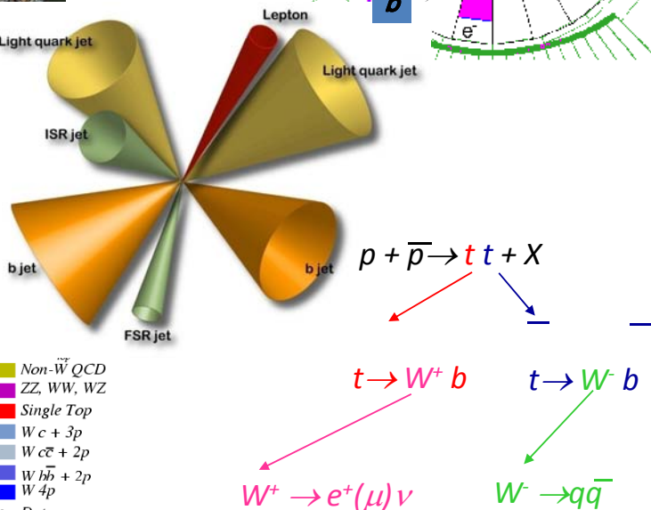
CDF Run II Preliminary 681 pb -1
