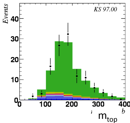
CDF Run II Preliminary 681 pb -1
