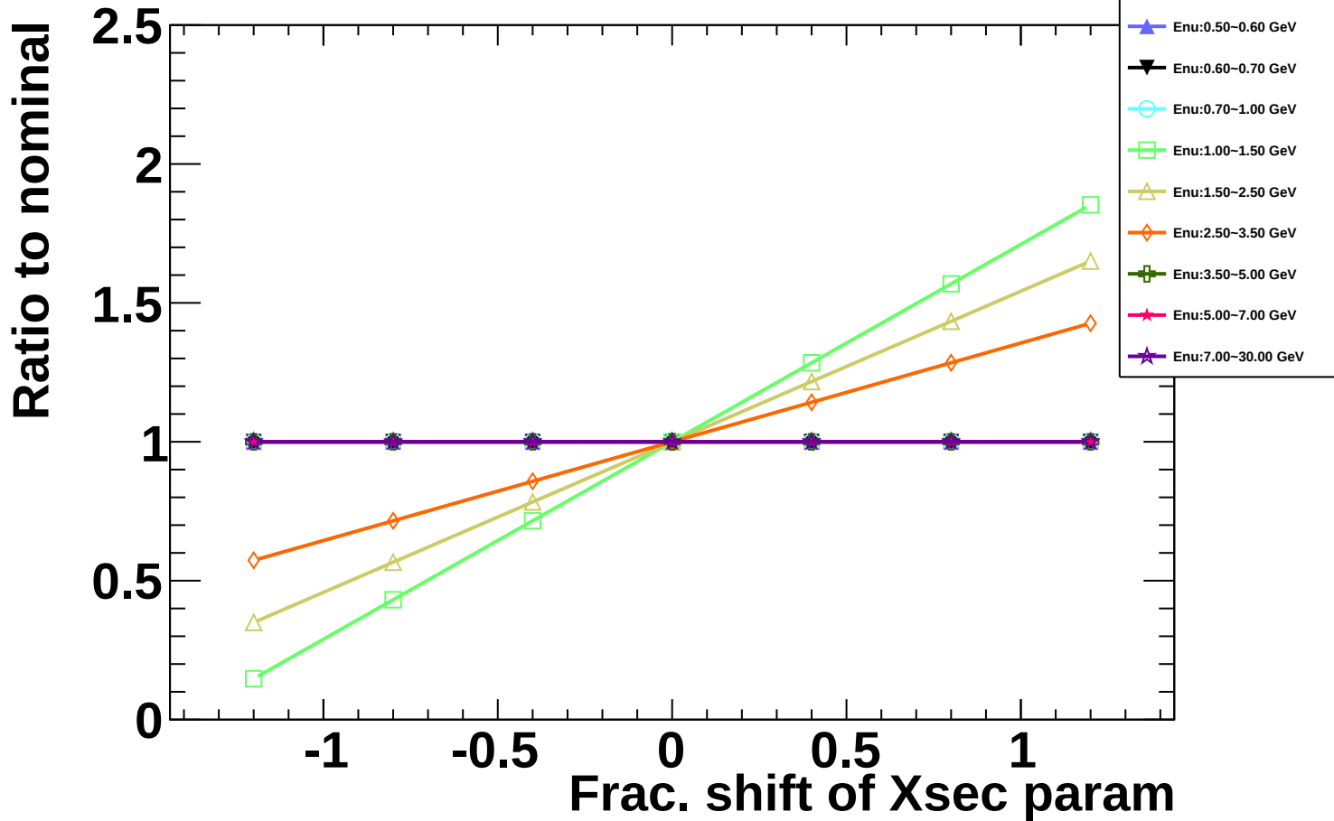
numubar ccothshp ccoth Erec:0.95~1.00 GeV
