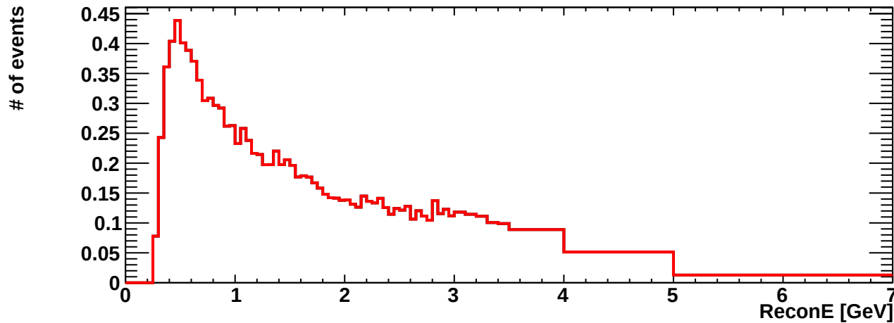
erec_int_numu_ccpi
