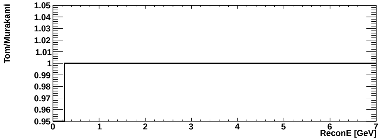
erec_int_numu_ccpi
