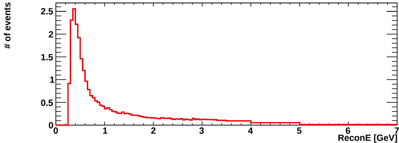
erec_int_numu_ccpi
