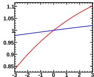
Enu=0.40-0.50GeV, Erec=0.45-0.50GeV (Red:Murakami, Blue:Tom)
