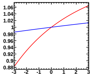
Enu=0.40-0.50GeV, Erec=0.55-0.60GeV (Red:Murakami, Blue:Tom)
