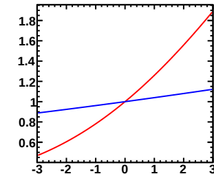
Enu=2.50-3.50GeV, Erec=0.35-0.40GeV (Red:Murakami, Blue:Tom)
