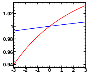
Enu=0.40-0.50GeV, Erec=0.30-0.35GeV (Red:Murakami, Blue:Tom)
