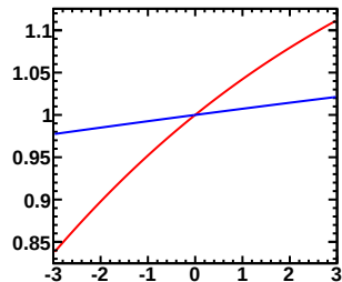
Enu=1.00-1.50GeV, Erec=0.00-0.30GeV (Red:Murakami, Blue:Tom)
