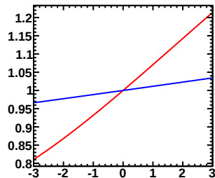
Enu=1.00-1.50GeV, Erec=1.80-1.90GeV (Red-Murakami, Blue-Tom)
