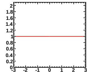
Enu=5.00-7.00GeV, Erec=0.50-0.55GeV (Red:Murakami, Blue:Tom)
