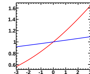
Enu=2.50-3.50GeV, Erec=0.75-0.80GeV (Red:Murakami, Blue:Tom)
