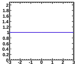
Enu=0.40-0.50GeV, Erec=0.40-0.45GeV (Red:Murakami, Blue:Tom)
