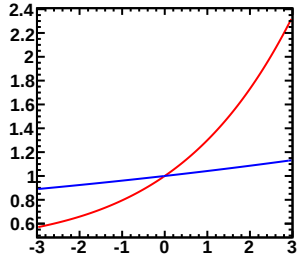
Enu=7.00-30.00GeV, Erec=10.00-30.00GeV (Red:Murakami, Blue:Tom)
