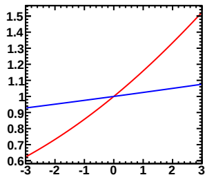
Enu=3.50-5.00GeV, Erec=2.60-2.70GeV (Red-Murakami, Blue-Tom)
