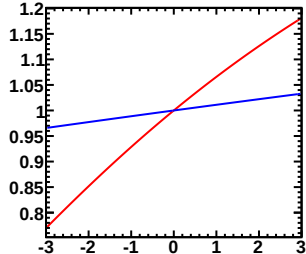
Enu=1.00-1.50GeV, Erec=0.70-0.75GeV (Red-Murakami, Blue-Tom)
