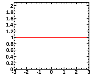
Enu=7.00-30.00GeV, Erec=0.50-0.55GeV (Red:Murakami, Blue:Tom)
