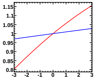
Enu=0.70-1.00GeV, Erec=0.80-0.85GeV (Red-Murakami, Blue-Tom)
