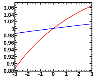
Enu=0.60-0.70GeV, Erec=0.00-0.30GeV (Red:Murakami, Blue:Tom)
