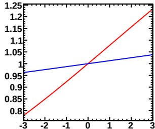
Enu=1.00-1.50GeV, Erec=1.40-1.50GeV (Red:Murakami, Blue:Tom)
