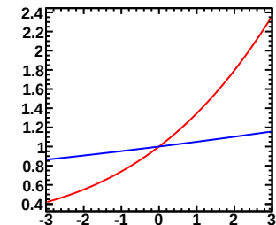
Enu=5.00-7.00GeV, Erec=2.70-2.80GeV (Red:Murakami, Blue:Tom)
