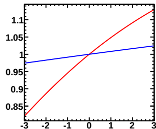
Enu=0.60-0.70GeV, Erec=0.55-0.60GeV (Red:Murakami, Blue:Tom)
