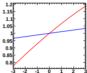
Enu=0.70-1.00GeV, Erec=0.85-0.90GeV (Red:Murakami, Blue:Tom)
