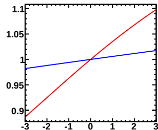
Enu=0.60-0.70GeV, Erec=0.65-0.70GeV (Red:Murakami, Blue:Tom)
