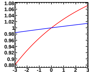
Enu=0.60-0.60GeV, Erec=0.35-0.40GeV (Red:Murakami, Blue:Tom)
