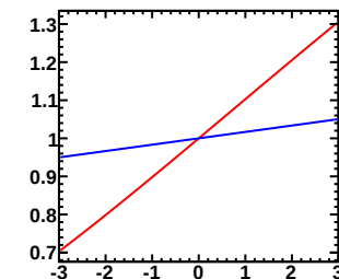
Enu=1.50-2.50GeV, Erec=0.75-0.80GeV (Red:Murakami, Blue:Tom)
