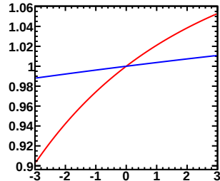
Enu=0.50-0.60GeV, Erec=0.00-0.30GeV (Red:Murakami, Blue:Tom)
