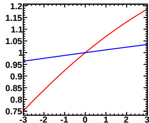
Enu=0.50-0.60GeV, Erec=0.55-0.60GeV (Red:Murakami, Blue:Tom)
