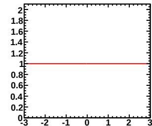
Enu=7.00-30.00GeV, Erec=0.00-0.30GeV (Red:Murakami, Blue:Tom)
