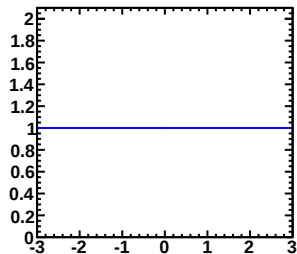
Enu=0.70-1.00GeV, Erec=1.00-1.10GeV (Red-Murakami, Blue-Tom)
