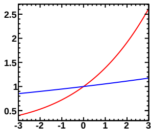
Enu=5.00-7.00GeV, Erec=2.60-2.70GeV (Red-Murakami, Blue-Tom)
