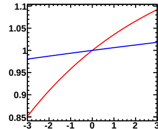
Enu=0.60-0.70GeV, Erec=0.35-0.40GeV (Red:Murakami, Blue:Tom)
