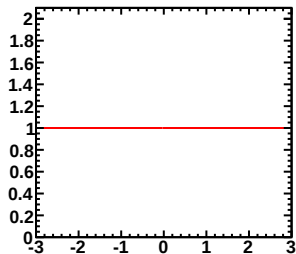
Enu=1.00-1.50GeV, Erec=2.60-2.70GeV (Red-Murakami, Blue-Tom)
