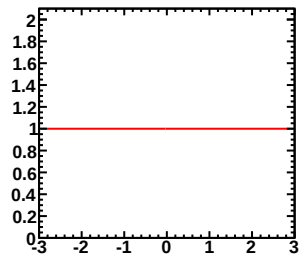
Enu=0.00-0.40GeV, Erec=0.30-0.35GeV (Red:Murakami, Blue:Tom)
