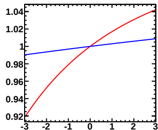
Enu=0.40-0.50GeV, Erec=0.35-0.40GeV (Red:Murakami, Blue:Tom)
