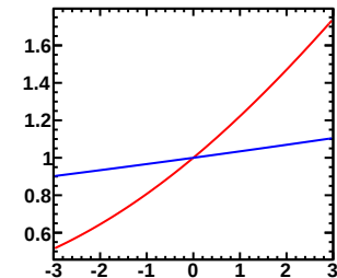
Enu=2.50-3.50GeV, Erec=0.50-0.55GeV (Red:Murakami, Blue:Tom)
