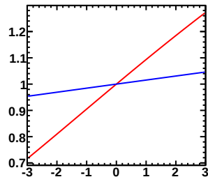
Enu=2.00-2.50GeV, Erec=0.95-1.00GeV (Red:Murakami, Blue:Tom)
