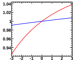
Enu=0.50-0.60GeV, Erec=0.65-0.70GeV (Red:Murakami, Blue:Tom)
