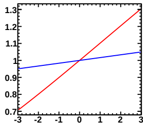
Enu=3.50-5.00GeV, Erec=2.80-2.90GeV (Red:Murakami, Blue:Tom)
