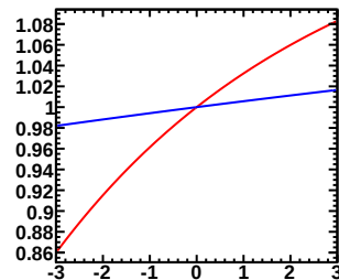
Enu=0.60-0.70GeV, Erec=0.30-0.35GeV (Red:Murakami, Blue:Tom)
