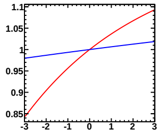
Enu=0.40-0.50GeV, Erec=0.85-0.90GeV (Red:Murakami, Blue:Tom)
