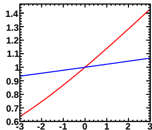
Enu=2.50-3.00GeV, Erec=0.95-1.00GeV (Red:Murakami, Blue:Tom)
