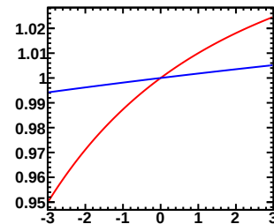
Enu=0.60-0.70GeV, Erec=0.75-0.80GeV (Red:Murakami, Blue:Tom)
