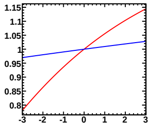
Enu=0.70-1.00GeV, Erec=1.50-1.60GeV (Red:Murakami, Blue:Tom)
