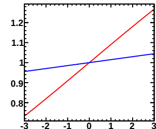
Enu=1.50-2.50GeV, Erec=0.45-0.50GeV (Red:Murakami, Blue:Tom)
