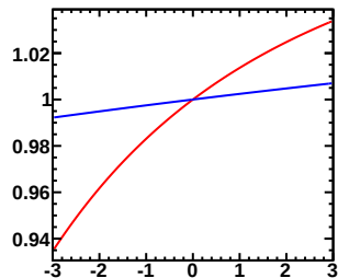
Enu=0.40-0.50GeV, Erec=0.50-0.55GeV (Red:Murakami, Blue:Tom)
