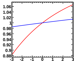
Enu=0.50-0.60GeV, Erec=0.30-0.35GeV (Red:Murakami, Blue:Tom)
