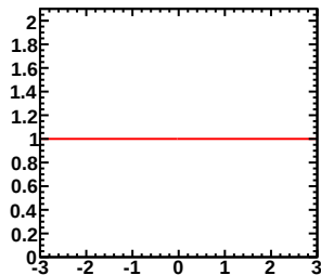
Enu=7.00-30.00GeV, Erec=2.60-2.70GeV (Red-Murakami, Blue-Tom)
