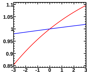
Enu=0.60-0.70GeV, Erec=0.45-0.50GeV (Red:Murakami, Blue:Tom)
