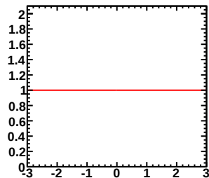
Enu=0.80-1.00GeV, Erec=0.95-1.00GeV (Red:Murakami, Blue:Tom)
