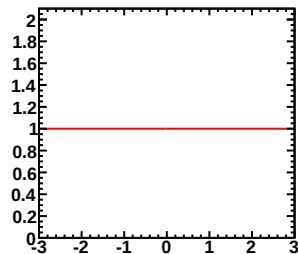
Enu=0.40-0.50GeV, Erec=1.80-1.90GeV (Red-Murakami, Blue-Tom)
