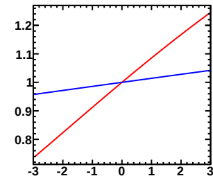
Enu=1.50-2.50GeV, Erec=0.50-0.55GeV (Red:Murakami, Blue:Tom)
