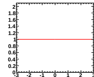
Enu=7.00-30.00GeV, Erec=0.75-0.80GeV (Red:Murakami, Blue:Tom)
