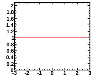
Enu=2.50-3.50GeV, Erec=0.00-0.30GeV (Red:Murakami, Blue:Tom)
