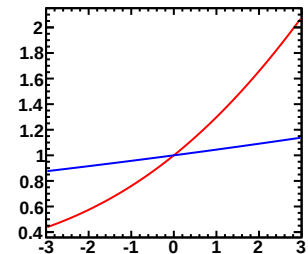
Enu=3.50-5.00GeV, Erec=0.80-0.85GeV (Red-Murakami, Blue-Tom)
