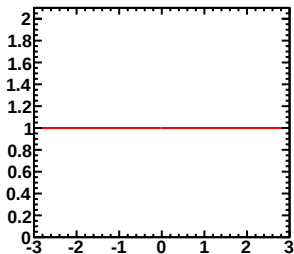
Enu=1.00-1.50GeV, Erec=2.50-2.60GeV (Red:Murakami, Blue:Tom)
