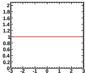
Enu=0.70-1.00GeV, Erec=2.60-2.70GeV (Red-Murakami, Blue-Tom)
