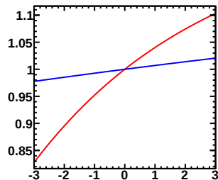
Enu=0.50-0.60GeV, Erec=0.50-0.55GeV (Red:Murakami, Blue:Tom)
