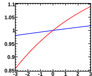
Enu=0.60-0.70GeV, Erec=0.40-0.45GeV (Red:Murakami, Blue:Tom)
