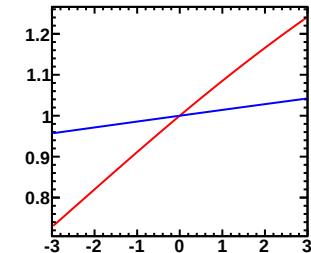
Enu=1.50-2.50GeV, Erec=0.35-0.40GeV (Red:Murakami, Blue:Tom)
