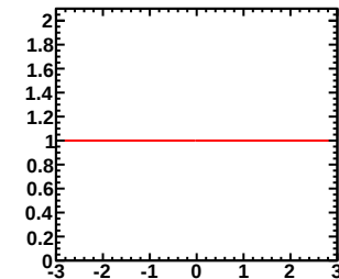
Enu=2.50-3.50GeV, Erec=0.30-0.35GeV (Red:Murakami, Blue:Tom)
