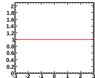
Enu=7.00-30.00GeV, Erec=0.45-0.50GeV (Red:Murakami, Blue:Tom)
