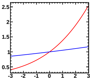
Enu=5.00-7.00GeV, Erec=2.50-2.60GeV (Red:Murakami, Blue:Tom)
