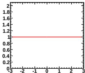
Enu=0.40-0.50GeV, Erec=2.60-2.70GeV (Red-Murakami, Blue-Tom)
