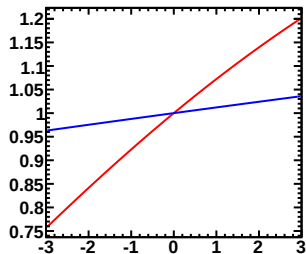
Enu=1.50-2.00GeV, Erec=0.95-1.00GeV (Red:Murakami, Blue:Tom)
