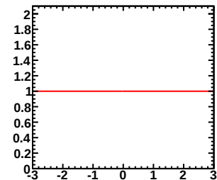
Enu=0.40-0.50GeV, Erec=0.80-0.85GeV (Red-Murakami, Blue-Tom)
