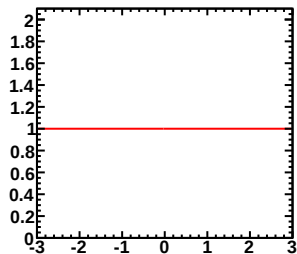
Enu=0.50-0.60GeV, Erec=1.70-1.80GeV (Red:Murakami, Blue:Tom)
