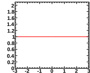
Enu=7.00-30.00GeV, Erec=0.35-0.40GeV (Red:Murakami, Blue:Tom)
