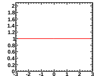
Enu=1.00-1.50GeV, Erec=2.70-2.80GeV (Red:Murakami, Blue:Tom)
