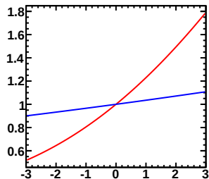
Enu=3.50-5.00GeV, Erec=1.80-1.90GeV (Red-Murakami, Blue-Tom)
