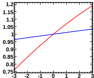
Enu=1.00-1.50GeV, Erec=0.80-0.85GeV (Red-Murakami, Blue-Tom)
