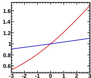
Enu=1.50-2.50GeV, Erec=2.60-2.70GeV (Red-Murakami, Blue-Tom)
