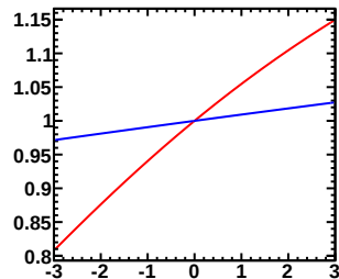
Enu=1.50-2.50GeV, Erec=0.30-0.35GeV (Red:Murakami, Blue:Tom)
