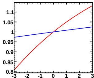
Enu=0.70-1.00GeV, Erec=0.40-0.45GeV (Red:Murakami, Blue:Tom)
