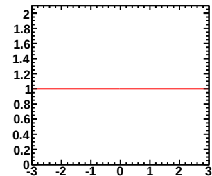
Enu=5.00-7.00GeV, Erec=0.80-0.85GeV (Red-Murakami, Blue-Tom)
