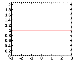
Enu=5.00-7.00GeV, Erec=0.85-0.90GeV (Red:Murakami, Blue:Tom)
