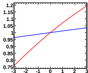
Enu=1.00-1.50GeV, Erec=0.65-0.70GeV (Red:Murakami, Blue:Tom)
