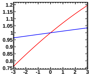
Enu=1.00-1.50GeV, Erec=0.90-0.95GeV (Red:Murakami, Blue:Tom)
