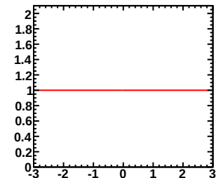
Enu=5.00-7.00GeV, Erec=0.45-0.50GeV (Red:Murakami, Blue:Tom)
