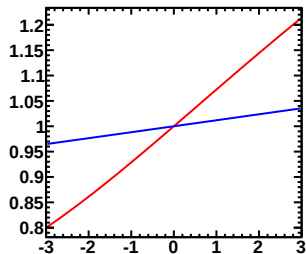
Enu=1.00-1.50GeV, Erec=0.95-1.00GeV (Red:Murakami, Blue:Tom)
