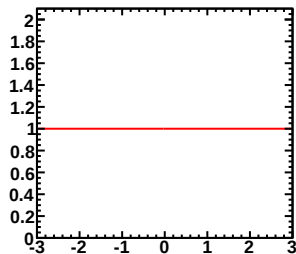
Enu=0.60-0.60GeV, Erec=3.00-3.50GeV (Red:Murakami, Blue:Tom)
