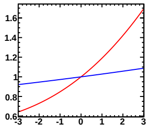
Enu=3.50-5.00GeV, Erec=1.00-1.10GeV (Red-Murakami, Blue-Tom)
