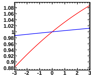
Enu=1.50-2.50GeV, Erec=0.00-0.30GeV (Red:Murakami, Blue:Tom)
