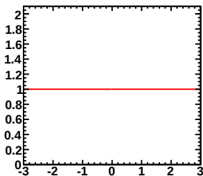
Enu=5.00-7.00GeV, Erec=0.65-0.70GeV (Red:Murakami, Blue:Tom)
