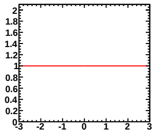
Enu=0.00-0.40GeV, Erec=1.00-1.10GeV (Red-Murakami, Blue-Tom)
