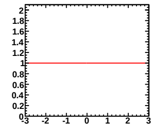
Enu=0.40-0.50GeV, Erec=2.70-2.80GeV (Red:Murakami, Blue:Tom)
