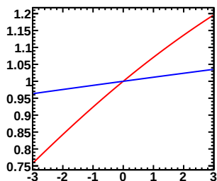
Enu=1.00-1.50GeV, Erec=0.60-0.65GeV (Red:Murakami, Blue:Tom)
