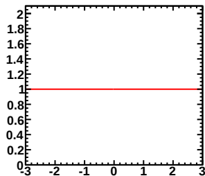
Enu=0.60-0.70GeV, Erec=2.60-2.70GeV (Red-Murakami, Blue-Tom)
