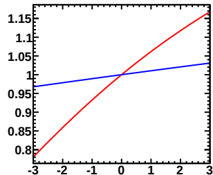
Enu=1.00-1.50GeV, Erec=0.35-0.40GeV (Red:Murakami, Blue:Tom)
