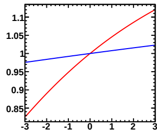
Enu=0.60-0.70GeV, Erec=0.50-0.55GeV (Red:Murakami, Blue:Tom)
