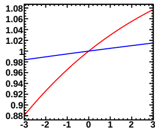
Enu=0.50-0.60GeV, Erec=0.45-0.50GeV (Red:Murakami, Blue:Tom)
