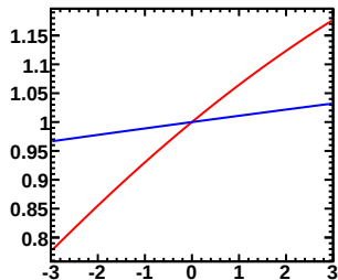
Enu=1.00-1.50GeV, Erec=0.40-0.45GeV (Red:Murakami, Blue:Tom)
