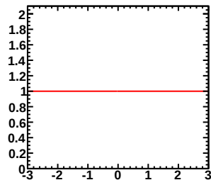
Enu=0.60-0.60GeV, Erec=4.00-5.00GeV (Red:Murakami, Blue:Tom)
