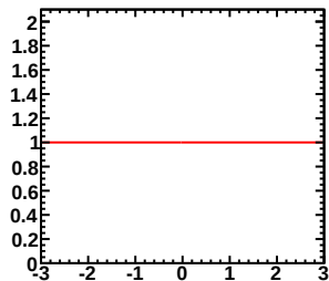
Enu=0.40-0.50GeV, Erec=5.00-7.00GeV (Red:Murakami, Blue:Tom)
