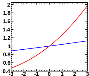
Enu=3.00-5.00GeV, Erec=0.95-1.00GeV (Red:Murakami, Blue:Tom)
