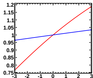
Enu=1.00-1.50GeV, Erec=0.85-0.90GeV (Red:Murakami, Blue:Tom)
