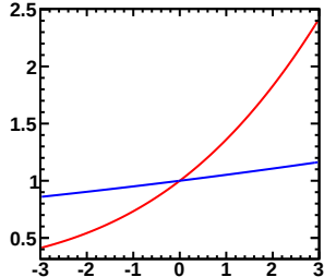
Enu=3.50-5.00GeV, Erec=10.00-30.00GeV (Red:Murakami, Blue:Tom)
