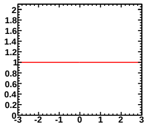
Enu=0.70-1.00GeV, Erec=10.00-30.00GeV (Red:Murakami, Blue:Tom)
