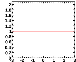
Enu=5.00-7.00GeV, Erec=0.35-0.40GeV (Red:Murakami, Blue:Tom)
