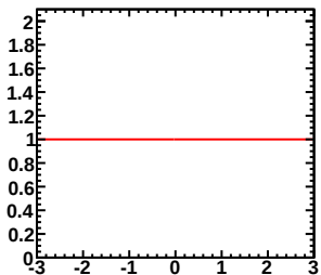
Enu=0.40-0.50GeV, Erec=2.80-2.90GeV (Red:Murakami, Blue:Tom)
