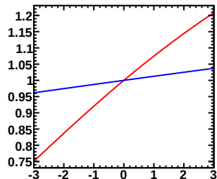
Enu=1.00-1.50GeV, Erec=0.45-0.50GeV (Red:Murakami, Blue:Tom)
