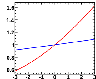
Enu=2.50-3.50GeV, Erec=0.45-0.50GeV (Red:Murakami, Blue:Tom)
