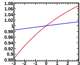
Enu=0.50-0.60GeV, Erec=0.40-0.45GeV (Red:Murakami, Blue:Tom)
