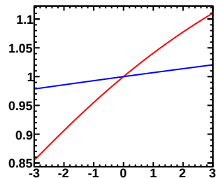
Enu=0.60-0.70GeV, Erec=0.60-0.65GeV (Red:Murakami, Blue:Tom)
