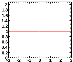
Enu=1.00-1.50GeV, Erec=2.30-2.40GeV (Red:Murakami, Blue:Tom)
