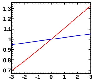
Enu=2.50-3.50GeV, Erec=2.60-2.70GeV (Red-Murakami, Blue-Tom)
