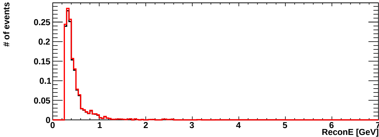
SK numu ncoth Recon. Energy Spectrum
