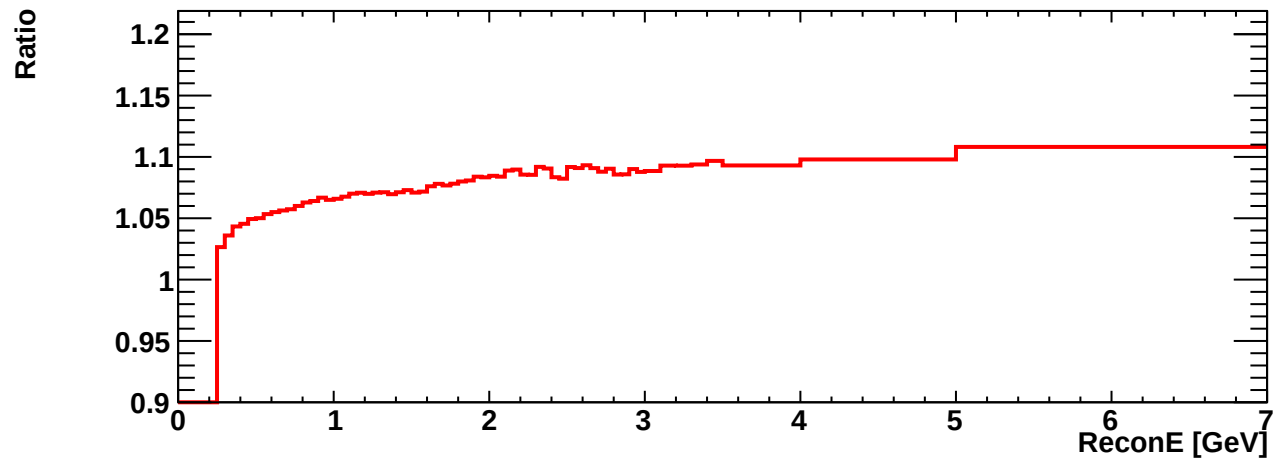
SK numu ccpi Recon. Energy Spectrum
