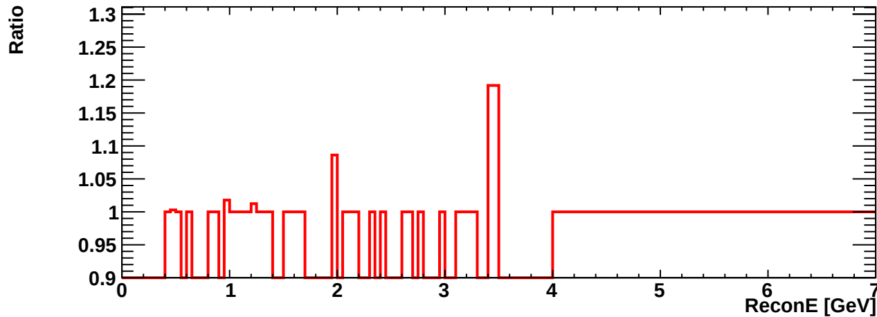
SK signue ccloth Recon. Energy Spectrum
