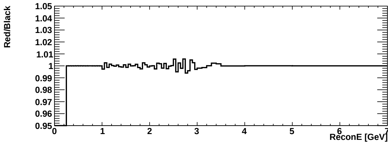
erec_int_numu_ccpi
