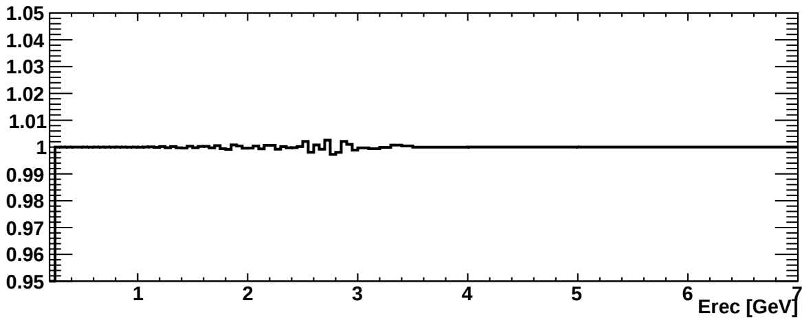
All flavors, All interactions
