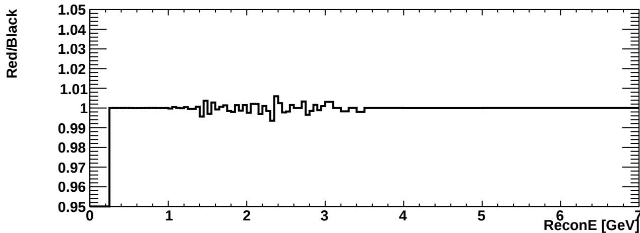
erec_int_numu_ccoth
