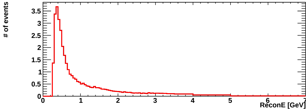
erec_int_numu_ccpi
