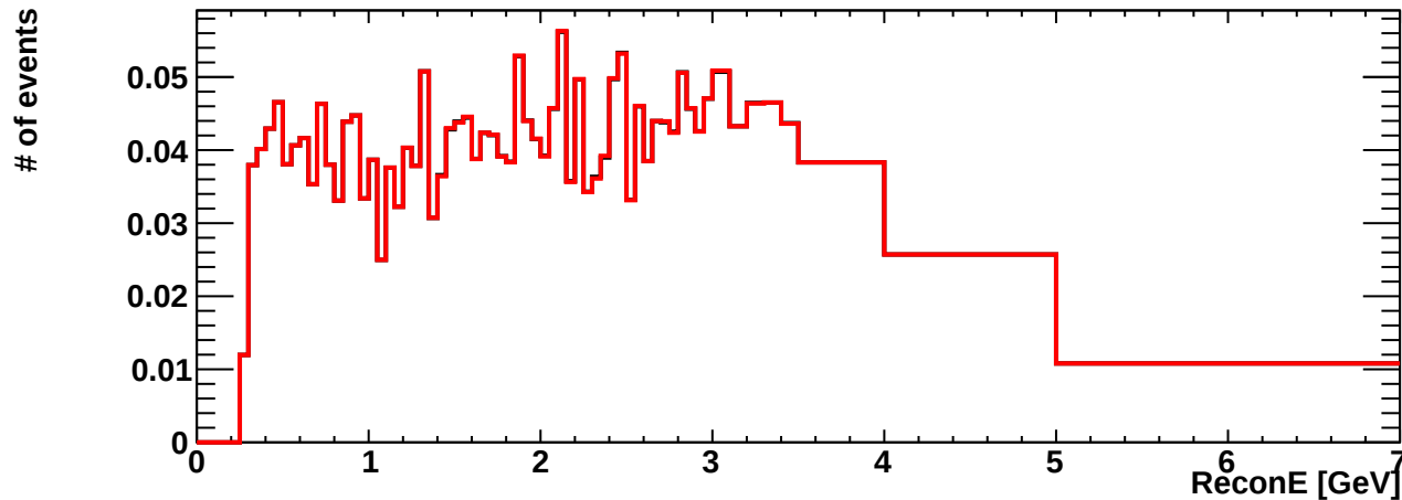
erec_int_numu_ccoth
