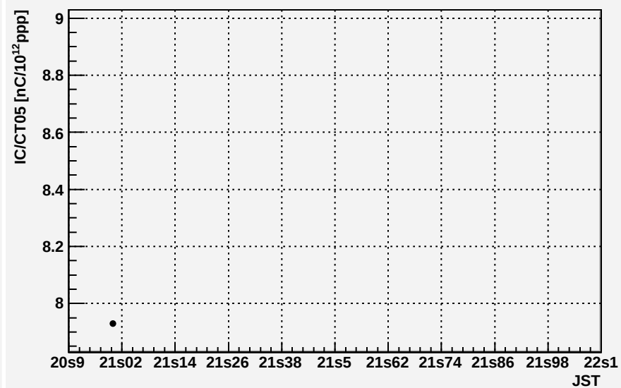
IC/CT05 history
