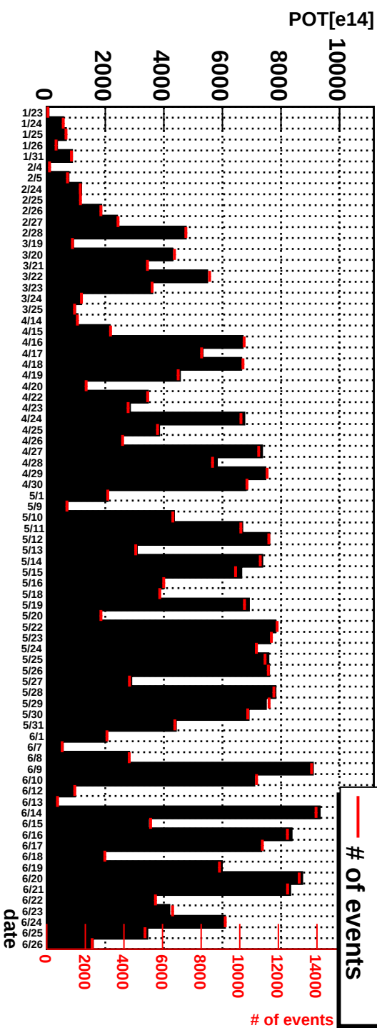
daily pot and number of neutrino candidates
