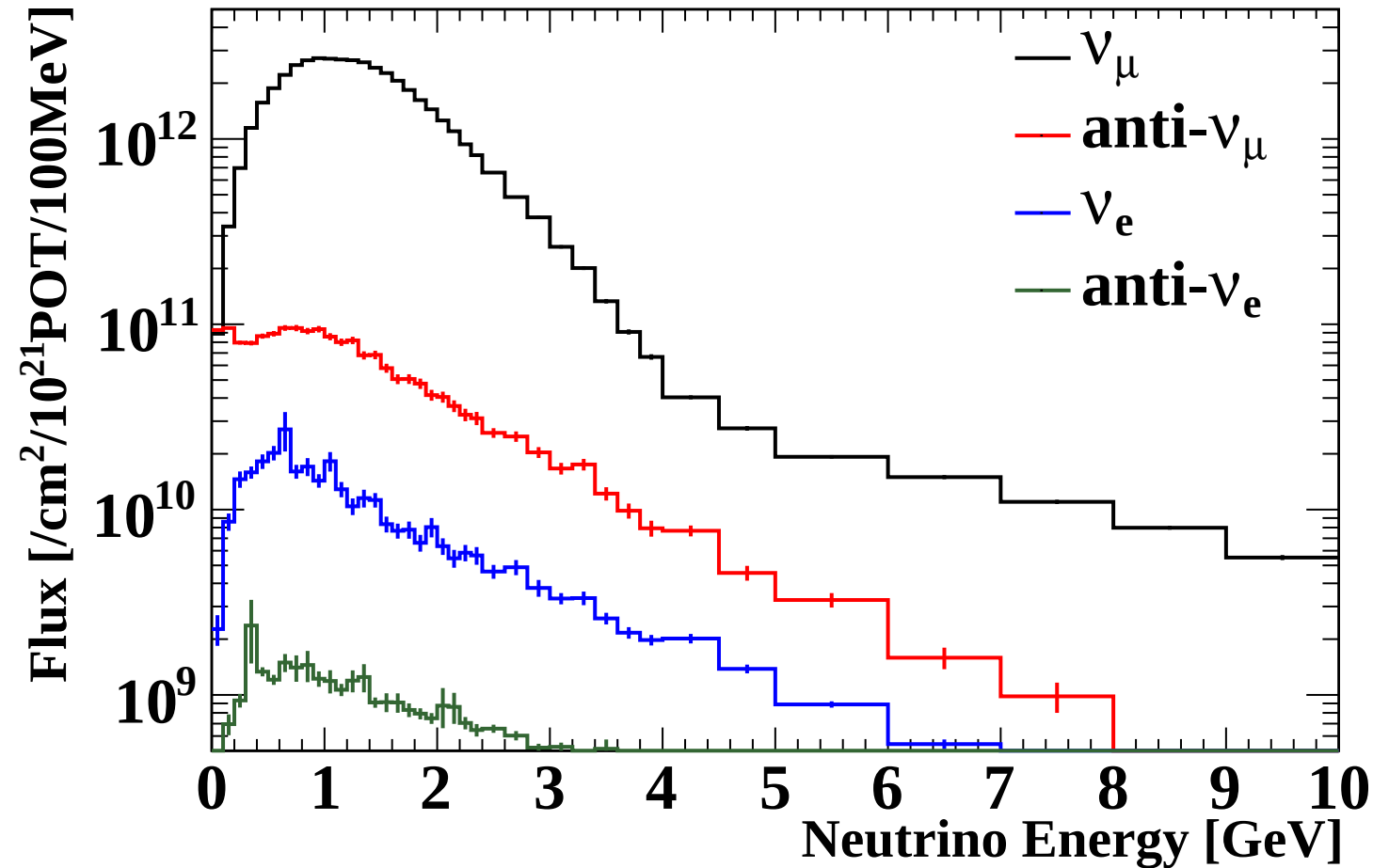
Neutrino Flux at module 3 (10d tuned-v2)
