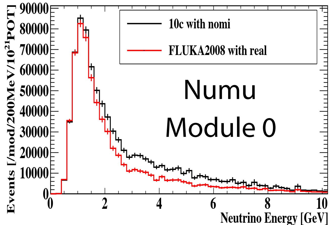
Neutrino energy spectrum (after neutrino selection) at module 0
