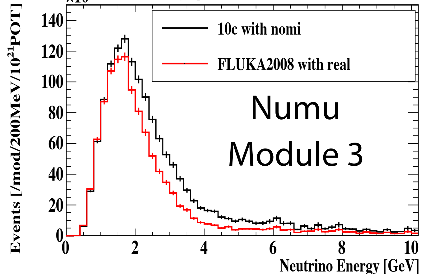
Neutrino energy spectrum (after neutrino selection) at module 3
