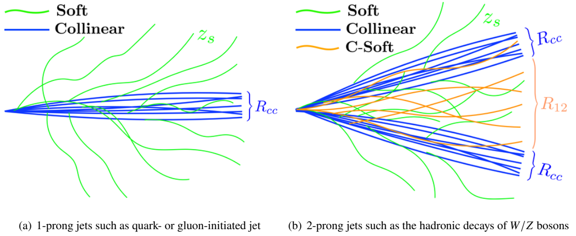
Figure 1.2: Schematic views of 1-prong jets (a) and 2-prong jets (b) [10]. Collinear (blue) and soft (green) radiations are illustrated. The angular size of the collinear radiation is R_{cc} and the p_T fraction of the soft radiation is z_s . For 2-prong jets, collinear-soft radiation emitted from the dipole formed by the two subjects represents the orange line. R_{12} represents the angle between these two subjects.
