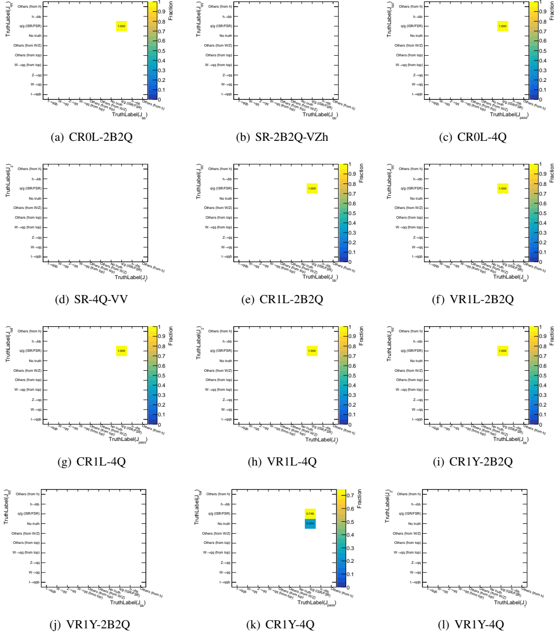
Figure K.2: Jet compositions of Z(\rightarrow ll)+\text{jets} events.
