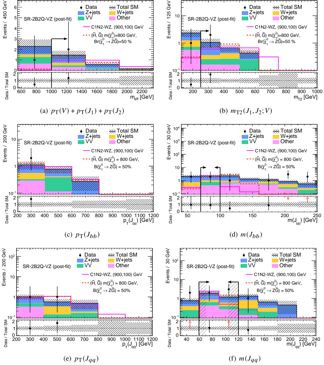
Figure 10.8: Distributions of p_T(V) + p_T(J_1) + p_T(J_2) (a), m_{T2}(J_1, J_2; V) (b), p_T(J_{bb}) (c), m(J_{bb}) (d), p_T(J_{qq}) (e), and m(J_{qq}) (f) in SR-2B2Q-VZ. “Other” includes VVV, t\bar{t} , t + X , t\bar{t} + X , Vh , \gamma + \text{jets} , and V\gamma .
