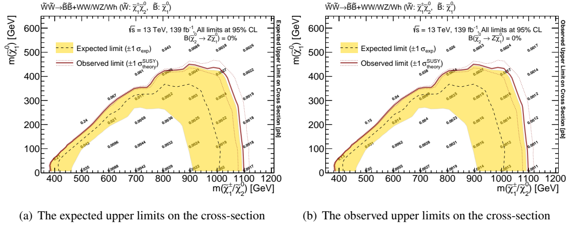
Figure S.21: Expected (a) and observed (b) upper limits on the cross-section with exclusion limits of the (\tilde{W}, \tilde{B}) model assuming \mathcal{B}(\tilde{\chi}_2^0 \rightarrow Z \tilde{\chi}_1^0) = 0\%
