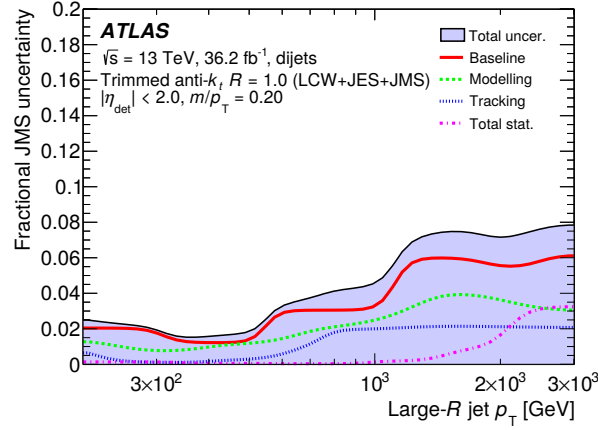
Figure 9.2: The uncertainty in the relative jet mass scale as a function of the large- R jet p_T with large- R jet m/p_T = 0.2 [109]. The baseline uncertainty represents the deviation of the double ratio from unity for PYTHIA 8. The modeling uncertainty represents the largest deviation from the unity of alternative MC generators. The tracking uncertainty represents the quadratic sum of the effect of three tracking variations.
