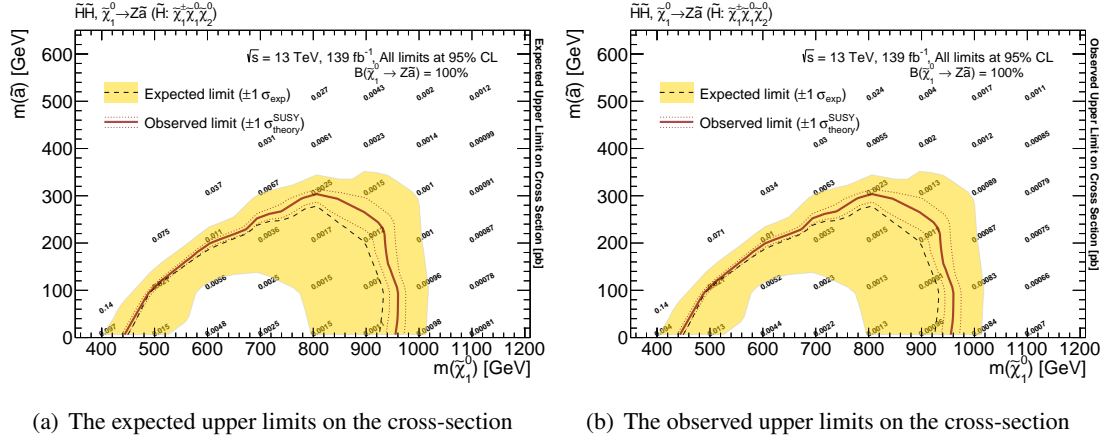
Figure S.41: Expected (a) and observed (b) upper limits on the cross-section with exclusion limits of the (\tilde{H}, \tilde{a}) model assuming \mathcal{B}(\tilde{\chi}_1^0 \rightarrow Z\tilde{a}) = 100\%
