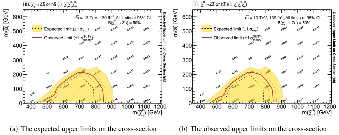
Figure S.43: Expected (a) and observed (b) upper limits on the cross-section with exclusion limits of the (\tilde{H}, \tilde{a}) model assuming \mathcal{B}(\tilde{\chi}_1^0 \rightarrow Z\tilde{a}) = 50\%
