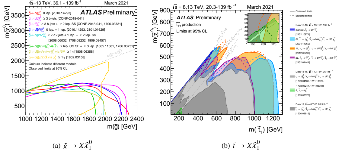
Figure 2.4: The exclusion limits at 95% C.L. for gluino ( \tilde{g} ) production (a) and stop ( \tilde{t} ) production (b), obtained in the simplified model using 36.1-139 \text{fb}^{-1} of pp -collision in Run-2 with ATLAS detector [29]. The horizontal axis represents \tilde{g} or \tilde{t} mass, and the vertical axis represents the lightest neutralino mass ( m(\tilde{\chi}_1^0) ). The regions inside (lower left side of) the contours are excluded (a), and the colored region is excluded (b).
