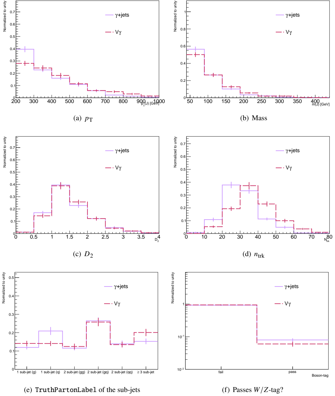
Figure O.4: The kinematic distributions of large- R jets which originate from quarks or gluons with Precut1Y2B2Q in various physics processes. The same descriptions as Figure 8.21 are applied.
