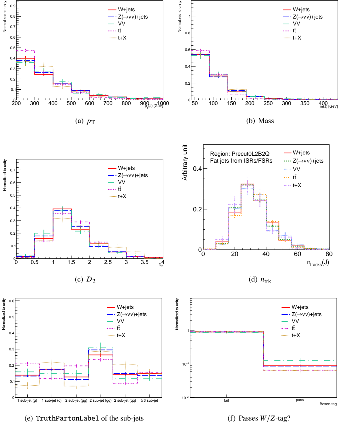
Figure O.1: The kinematic distributions of large- R jets which originate from quarks or gluons with Precut0L2B2Q in various physics processes. The same descriptions as Figure 8.21 are applied.
