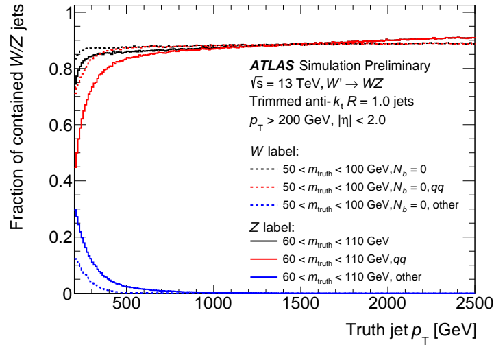
Figure E.1: Fraction of jets as a function of truth jet p_T matched to W (dashed lines) or Z bosons (solid lines) that pass the corresponding label criteria in a p_T flattened HVT W' samples [121]. The black lines represent the fractions after \Delta R -matching between truth bosons and truth jets, truth mass cuts, and ghost-associated b -hadron [129] requirements. The red lines show the fractions required to satisfy \Delta R -matching between truth jets and truth particles from hadronically decaying bosons, and the blue ones are not satisfied.
