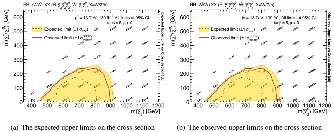
Figure S.34: Expected (a) and observed (b) upper limits on the cross-section with exclusion limits of the ( \tilde{H}, \tilde{W} ) model assuming \tan\beta = 5, \mu > 0 .
