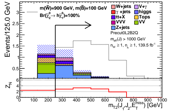
(b) m_{T2}(J_1, J_2; E_T^{\text{miss}}) in SR-2B2Q-Wh
