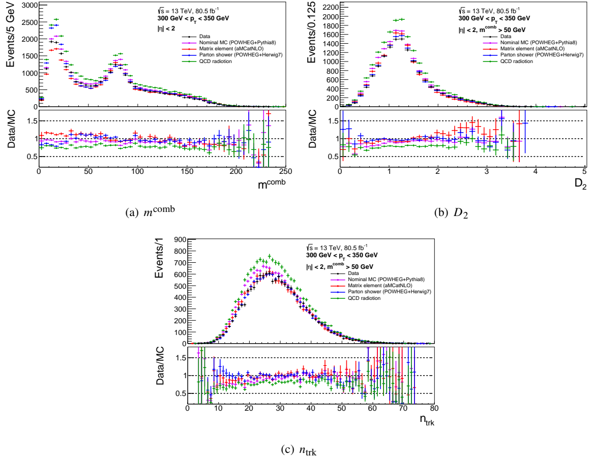
Figure G.6: Distributions of m^{\text{comb}} (a), D_2 (b), and n_{\text{trk}} (c) in data and MC samples with 300 \text{ GeV} < \text{jet } p_T < 350 \text{ GeV} . The black line represents data samples. Except for the black line, each color line represents MC expected distributions with different t\bar{t} MC samples (other samples are common). The violet line represents nominal MC sample, alternative MCs for the variation of matrix elements (red), parton shower (blue), and QCD radiation (green) are shown.
