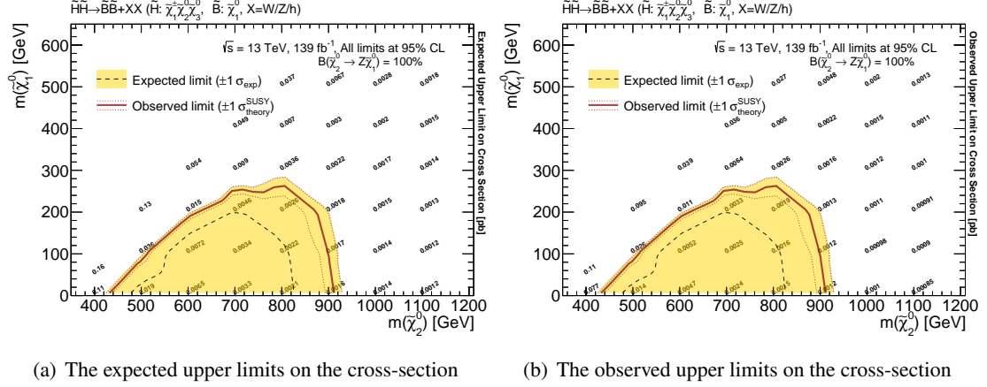
Figure S.22: Expected (a) and observed (b) upper limits on the cross-section with exclusion limits of the ( \tilde{H}, \tilde{B} ) model assuming \mathcal{B}(\tilde{\chi}_2^0 \rightarrow Z\tilde{\chi}_1^0) = 100\%
