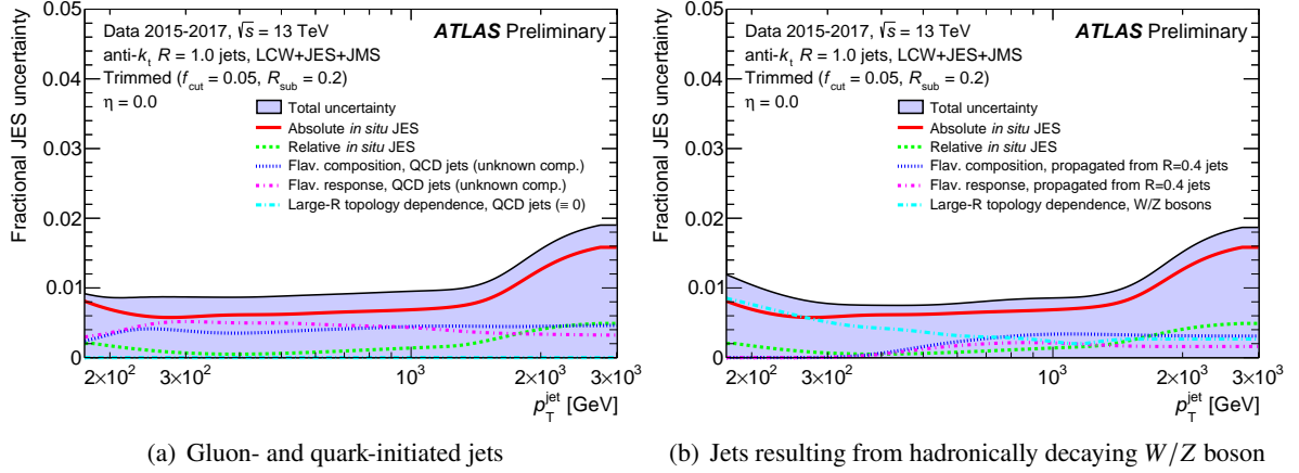
Figure 9.1: The uncertainty as a function of jet p_T of gluon- and quark-initiated jets (a) and jets resulting from hadronically decaying W/Z boson (b) [110]. Flavor uncertainties are propagated from small- R jets. “Relative in situ JES” are uncertainties from the \eta inter-calibration, and “Absolute in situ JES” includes all uncertainties of in-situ measurement in the central region. Total uncertainties are determined as the quadruple sum of each component.
