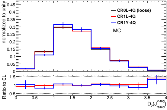
(c) D_2
