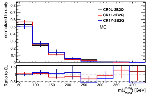
(b) mass
