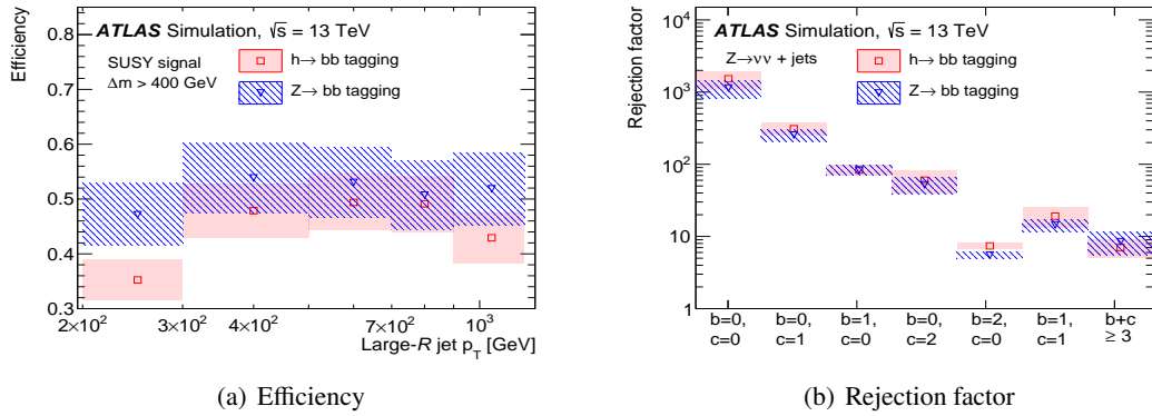
Figure 6.17: (a) Efficiency of h \rightarrow bb (red) and Z \rightarrow bb (blue) tagging efficiency by \tilde{\chi}_1^\pm \tilde{\chi}_2^0 signals. (b) Rejection factor (defined as the inverse of efficiency) [49]. The x -axis represents the number of b - or c -quark initiated sub-jets. The hashed bands represent the uncertainty, including the MC statistical uncertainty and the systematic uncertainties, such as the jet mass scale, the jet mass resolution, and the b -tagging uncertainties.
