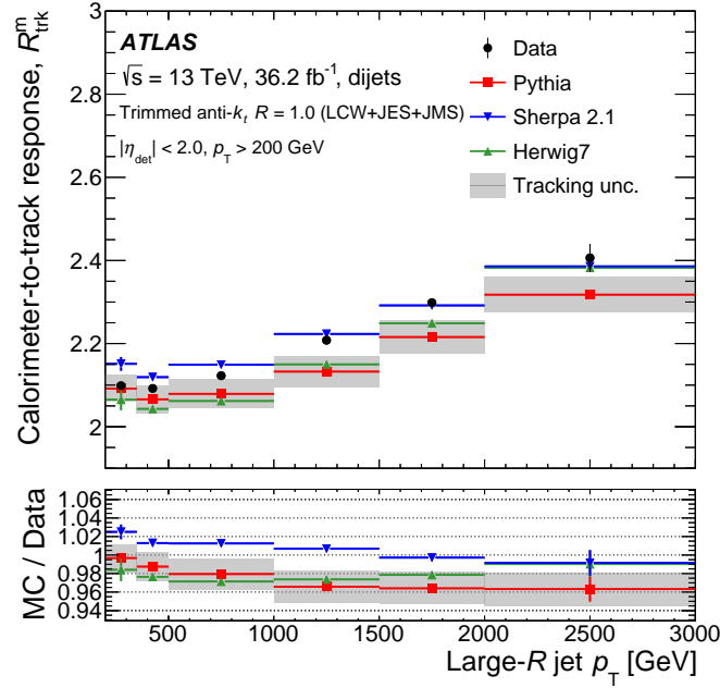
Figure 5.6: JMS in the R_{\text{trk}} method as a function of the large- R jet p_T [109]. Measurement of R_{\text{trk}}^m as a function of the large- R jet p_T with large- R jet m/p_T = 0.2 . Results using three different generators are shown. Tracking uncertainty for the default generator PYTHIA 8 is shown in the gray band. 5Reprinted from [109], Copyright 2019, The Author licensed under the CC-BY-4.0.
