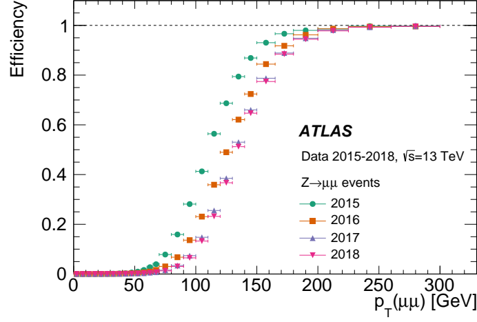
Figure 7.1: The lowest E_T^{\text{miss}} trigger efficiency combined L1 and HLT for the years 2015 to 2018 is shown as a function of the Z boson transverse momentum [142]. The events are taken from data with a Z \rightarrow \mu\mu selection. Muons are treated as invisible particles, and the transverse momentum of the di-muon system ( p_T(\mu\mu) ) is a proxy for E_T^{\text{miss}} . In all years, high efficiency is maintained at the high E_T^{\text{miss}} region ( E_T^{\text{miss}} \geq 200 GeV).
