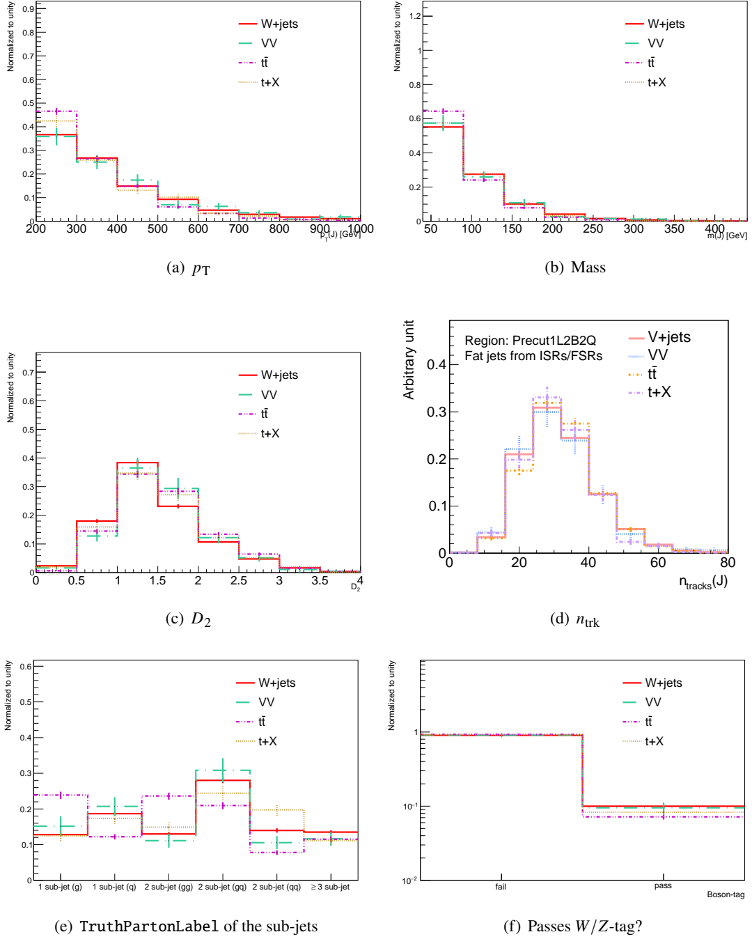
Figure O.3: The kinematic distributions of large- R jets which originate from quarks or gluons with Precut1L2B2Q in various physics processes. The same descriptions as Figure 8.21 are applied.
