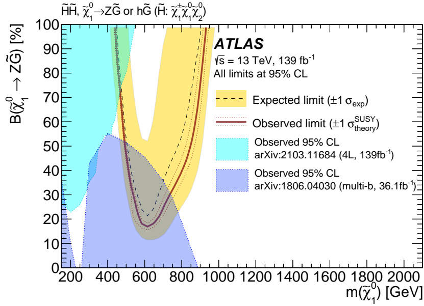
Figure 10.14: Expected (dashed black) and observed (solid red) exclusion limits for the (\tilde{H}, \tilde{G}) model at the 95% CL, as a function of the lightest neutralino mass m(\tilde{\chi}_1^0) and the branching ratio \mathcal{B}(\tilde{\chi}_1^0 \rightarrow Z\tilde{G}) = 1 - \mathcal{B}(\tilde{\chi}_1^0 \rightarrow h\tilde{G}) [49]. The exclusion limits from the previous ATLAS search using multi-lepton analysis [161] (cyan) and final states with multi- b analysis [162] (blue) are shown by the shades.
