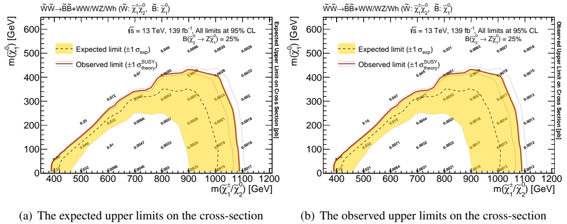
Figure S.20: Expected (a) and observed (b) upper limits on the cross-section with exclusion limits of the (\tilde{W}, \tilde{B}) model assuming \mathcal{B}(\tilde{\chi}_2^0 \rightarrow Z\tilde{\chi}_1^0) = 25\%
