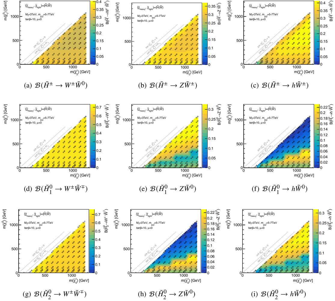
Figure C.15: Branching ratio of (a)(b)(c) charged higgsino (d)(e)(f) light neutral higgsino and (g)(h)(i) heavy neutral higgsino ( \tilde{H}_2^0 ) decaying wino light state with a into W/Z/h ( \tan \beta = 10, \mu < 0 ).
