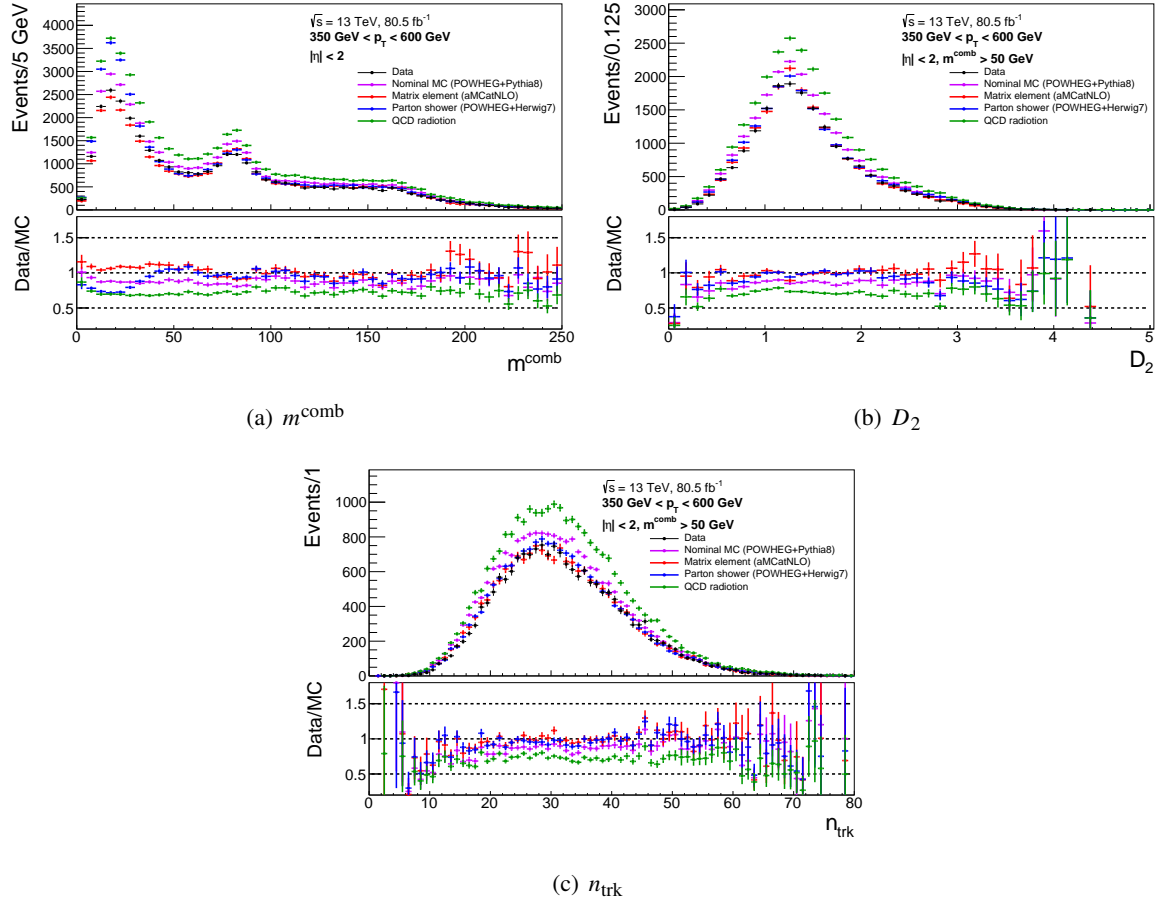
Figure G.7: Distributions of m^{\text{comb}} (a), D_2 (b), and n_{\text{trk}} (c) in data and MC samples with 350 \text{ GeV} < \text{jet } p_T < 600 \text{ GeV} . The black line represents data samples. Except for the black line, each color line represents MC expected distributions with different t\bar{t} MC samples (other samples are common). The violet line represents a nominal MC sample, alternative MCs for the variation of matrix elements (red), parton shower (blue), and QCD radiation (green) are shown.
