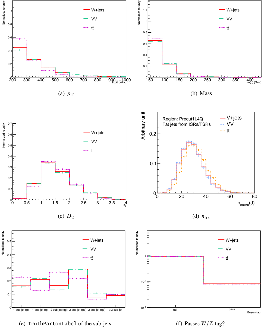
Figure O.2: The kinematic distributions of large- R jets which originate from quarkis or gluons with Precut1L4Q in various physics processes. The same descriptions as Figure 8.21 are applied.
