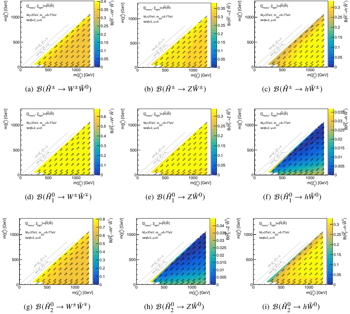
Figure C.9: Branching ratio of (a)(b)(c) charged higgsino (d)(e)(f) light neutral higgsino and (g)(h)(i) heavy neutral higgsino ( \tilde{H}_2^0 ) decaying wino light state with a into W/Z/h ( \tan\beta = 2 , \mu > 0 ).
