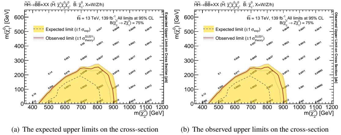
Figure S.23: Expected (a) and observed (b) upper limits on the cross-section with exclusion limits of the ( \tilde{H}, \tilde{B} ) model assuming \mathcal{B}(\tilde{\chi}_2^0 \rightarrow Z\tilde{\chi}_1^0) = 75\%
