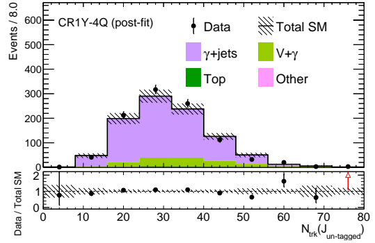
(e) n_{\text{trk}}(J_{\text{un-tagged}})
