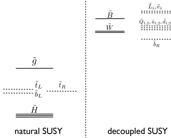
Figure 2.3: The mass spectra in the natural SUSY scenario [24]. Electroweak symmetry breaking constrains the superpartners on the left to be light. Other superpartners on the right can be heavy ( M \gg 1 TeV).
