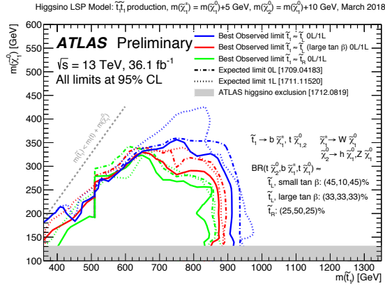
Figure 2.5: The exclusion limits at 95% C.L. for stop ( \tilde{t} ) production and higgsino ( \tilde{H} ) LSP model, obtained using 36.1 \text{fb}^{-1} of pp -collision in Run-2 with ATLAS detector [29]. The horizontal axis represents \tilde{t} mass, and the vertical axis represents the lightest neutral higgsino mass ( m(\tilde{\chi}_1^0) ). The regions inside (lower left side of) the contours are excluded. Only higgsino mass splitting among the higgsino mass eigenstates ( \tilde{\chi}_1^0, \tilde{\chi}_2^0, \tilde{\chi}_1^\pm ) is fixed. The stop can decay to the LSP via some processes, such as direct decay to the LSP ( \tilde{\chi}_1^0 ) with top quark or in two steps via chargino ( \tilde{\chi}_1^\pm ) or not the lightest neutralino ( \tilde{\chi}_2^0 ). This corresponding branching fraction depends on parameters, such as the stop left-right mixing and \tan\beta . Three results in different scenarios are described as different color lines.
