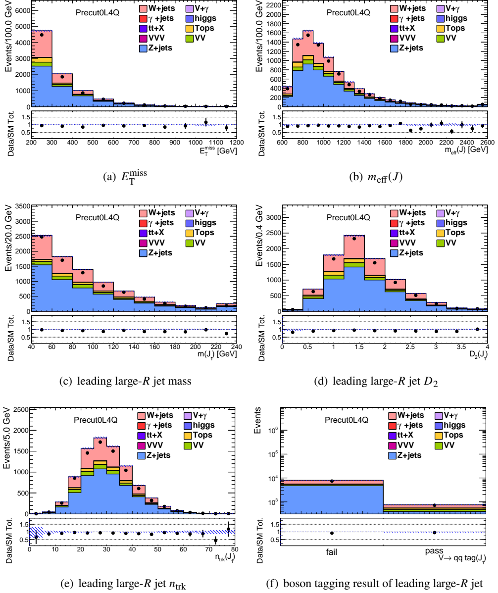
Figure I.1: Kinematic distributions of E_T^{\text{miss}} (a), m_{\text{eff}}(J) (b), and leading large- R jet mass (c), D_2 (d), n_{\text{trk}} (e), and boson tagging result (f) with Precut0L4Q selections.
