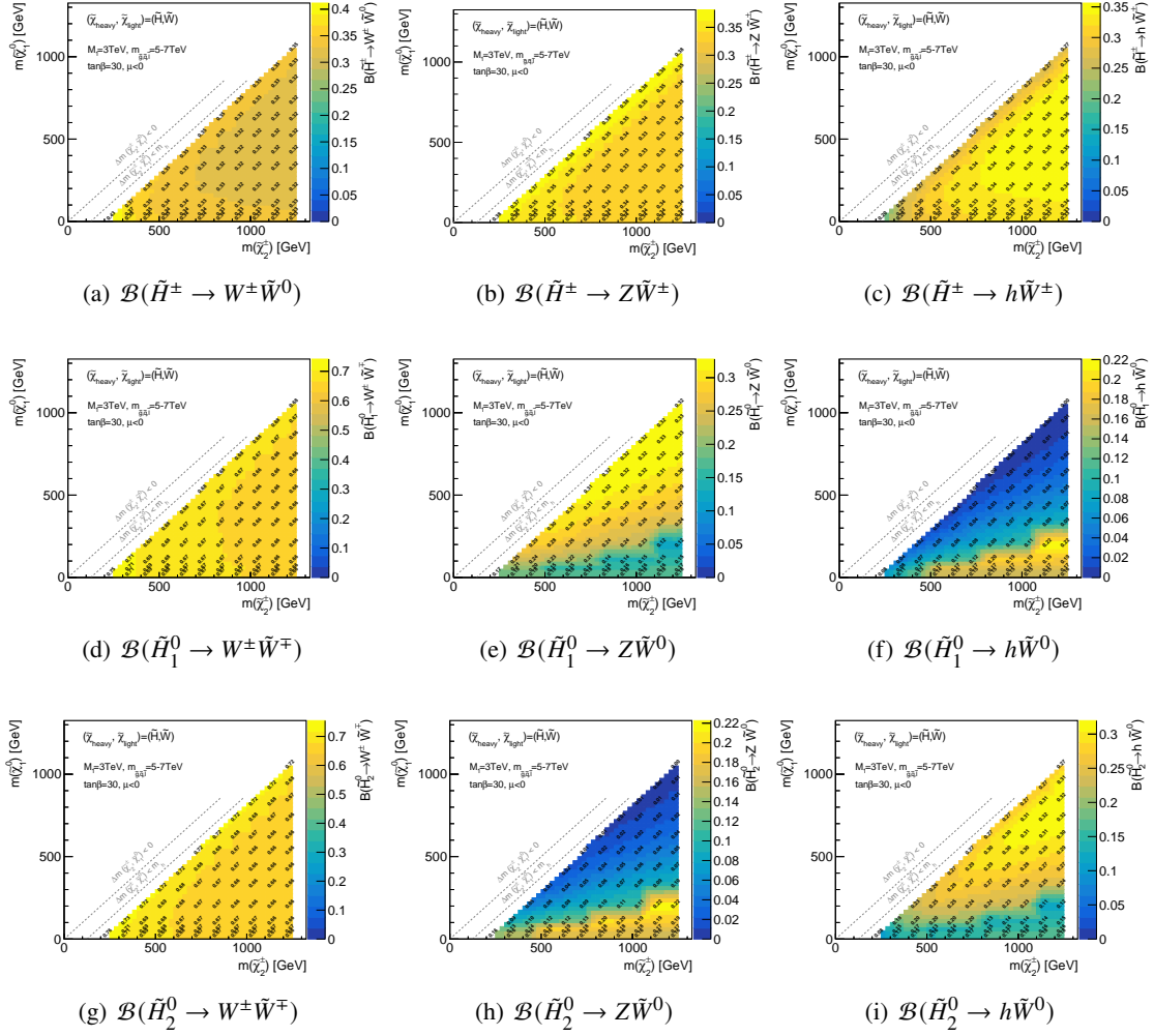
Figure C.16: Branching ratio of (a)(b)(c) charged higgsino (d)(e)(f) light neutral higgsino and (g)(h)(i) heavy neutral higgsino ( \tilde{H}_2^0 ) decaying wino light state with a into W/Z/h ( \tan \beta = 30, \mu < 0 ).
