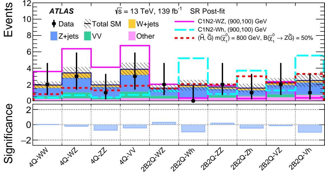
Figure 10.6: Comparison between the observed data and the post-fit SM background prediction in the SRs [49]. For the C1N2-WZ and C1N2-Wh models, the label (900, 100) GeV represents ( m(\tilde{\chi}_2^0) = 900 GeV, m(\tilde{\chi}_1^0) = 100 GeV). “Other” includes VVV , t\bar{t} , t + X , t\bar{t} + X , Vh , \gamma + \text{jets} , and V\gamma . The bottom panel shows the statistical significance of the discrepancy between the observed events and the expected SM backgrounds.
