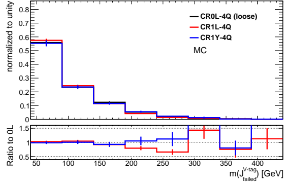
(b) mass
