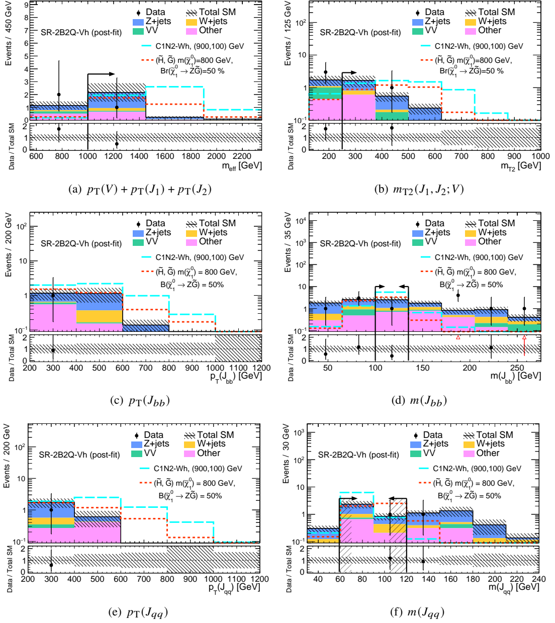
Figure 10.9: Distributions of p_T(V) + p_T(J_1) + p_T(J_2) (a), m_{T2}(J_1, J_2; V) (b), p_T(J_{bb}) (c), m(J_{bb}) (d), p_T(J_{qq}) (e), and m(J_{qq}) (f) in SR-2B2Q-Vh. “Other” includes VVV, t\bar{t} , t + X , t\bar{t} + X , Vh , \gamma + \text{jets} , and V\gamma .
