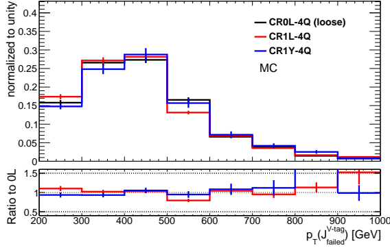
(a) p_T
