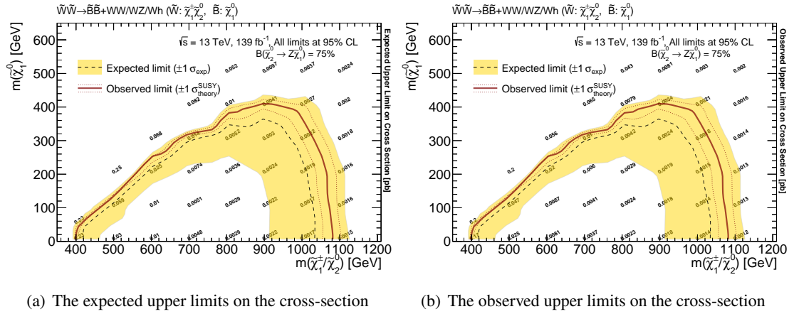
Figure S.18: Expected (a) and observed (b) upper limits on the cross-section with exclusion limits of the ( \tilde{W}, \tilde{B} ) model assuming \mathcal{B}(\tilde{\chi}_2^0 \rightarrow Z\tilde{\chi}_1^0) = 75\%
