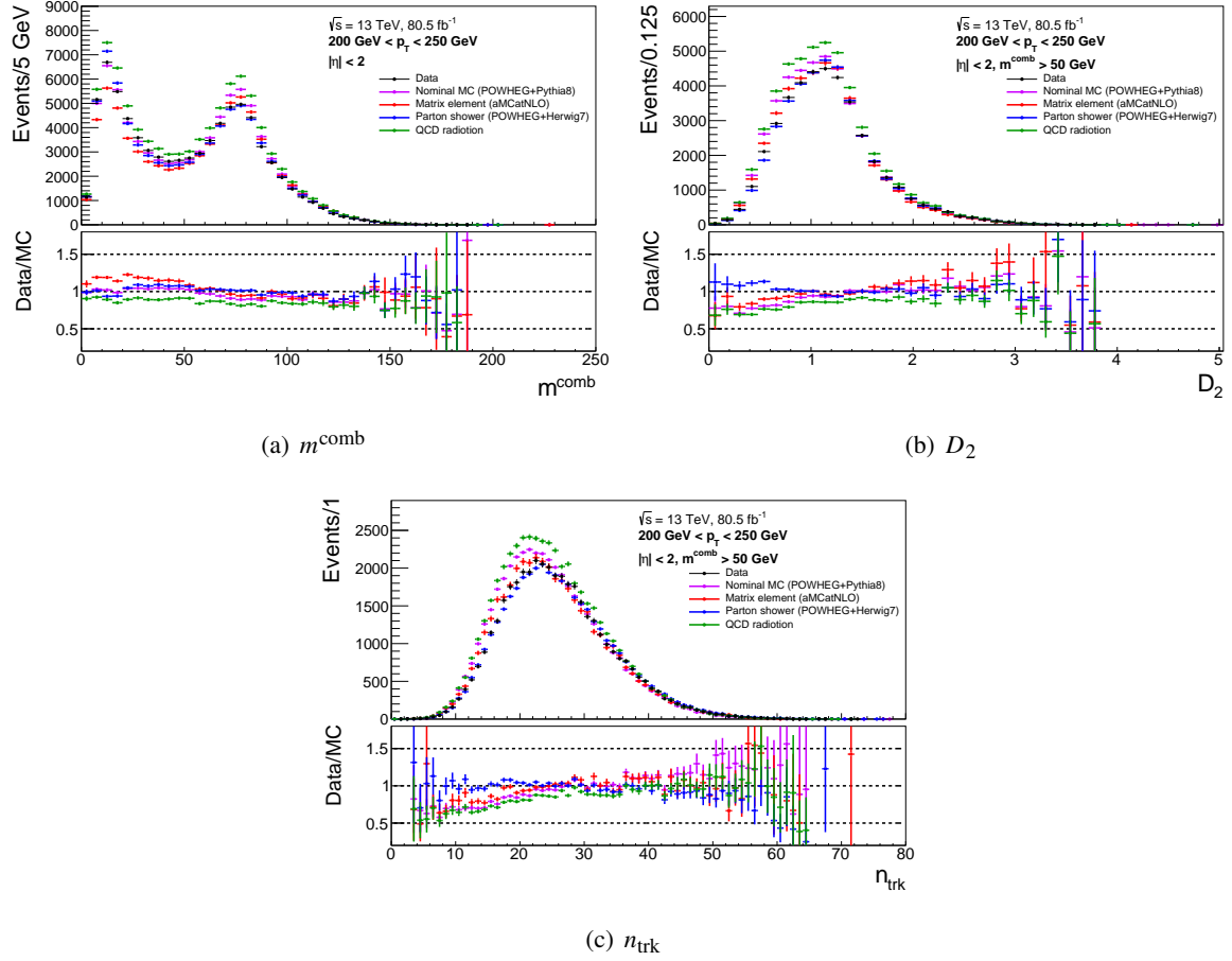
Figure G.4: Distributions of m^{\text{comb}} (a), D_2 (b), and n_{\text{trk}} (c) in data and MC samples with 200 \text{ GeV} < \text{jet } p_T < 250 \text{ GeV} . The black line represents data samples. Except for the black line, each color line represents MC expected distributions with different t\bar{t} MC samples (other samples are common). The violet line represents a nominal MC sample, alternative MCs for the variation of matrix elements (red), parton shower (blue), and QCD radiation (green) are shown.
