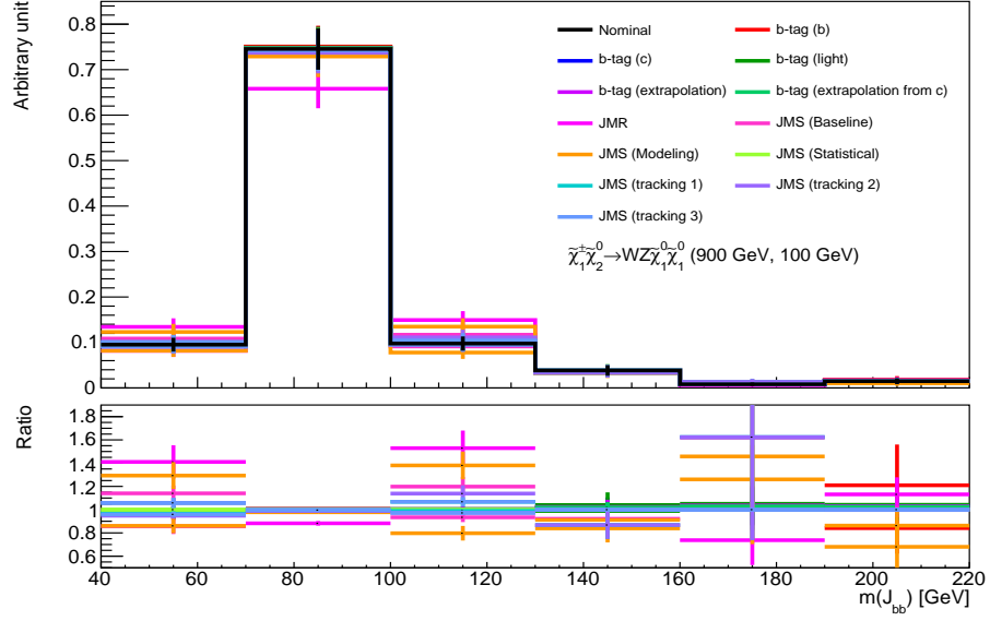
(a) C1N2-WZ
