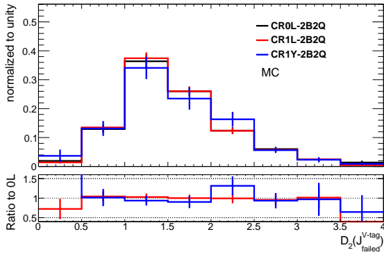
(c) D_2
