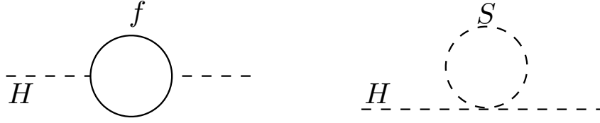
Figure 2.1: One-loop quantum corrections to the Higgs squared mass parameter m_H^2 , from Dirac fermion f (left) and scalar S (right).
