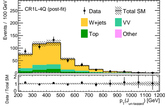
(b) p_T(J_{\text{un-tagged}})
