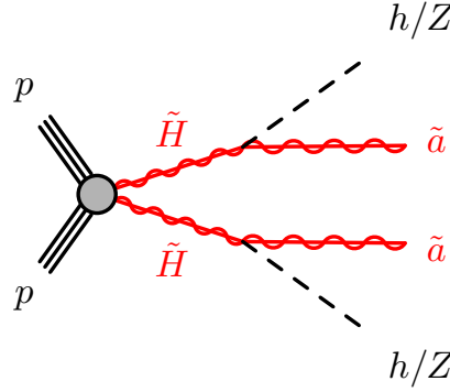
Figure 2.15: The diagram of (\tilde{H}, \tilde{a}) [49].
