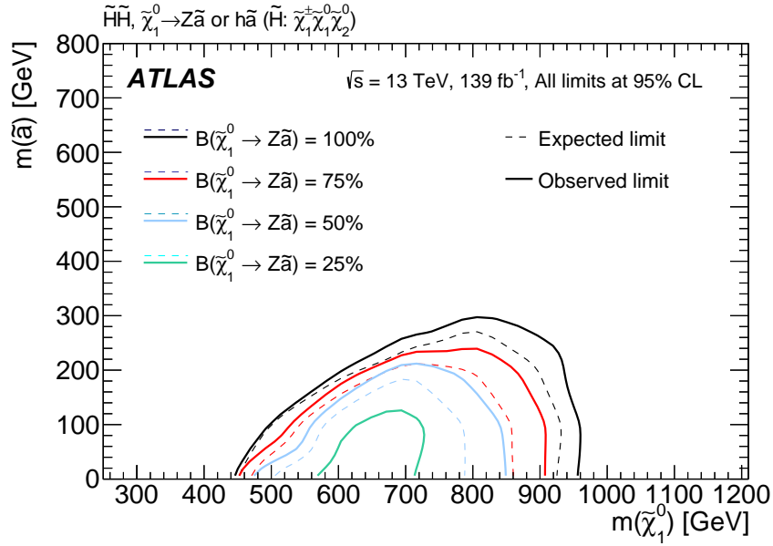
Figure 10.15: Expected (dashed lines) and observed (solid lines) limits with various \mathcal{B}(\tilde{\chi}_1^0 \rightarrow Z\tilde{a}) ( = 1 - \mathcal{B}(\tilde{\chi}_1^0 \rightarrow h\tilde{a}) ) hypothesis as a function of the lightest neutralino mass m(\tilde{\chi}_1^0) and the axino mass m(\tilde{a}) at the 95% CL [49]. There is no expected limit with \mathcal{B}(\tilde{\chi}_1^0 \rightarrow Z\tilde{a}) = 25\% because the CLs values of all the benchmark signal points in the (m(\tilde{\chi}_1^0), m(\tilde{a})) plane is less than 0.05.
