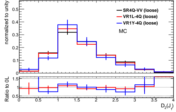
(b) D_2
