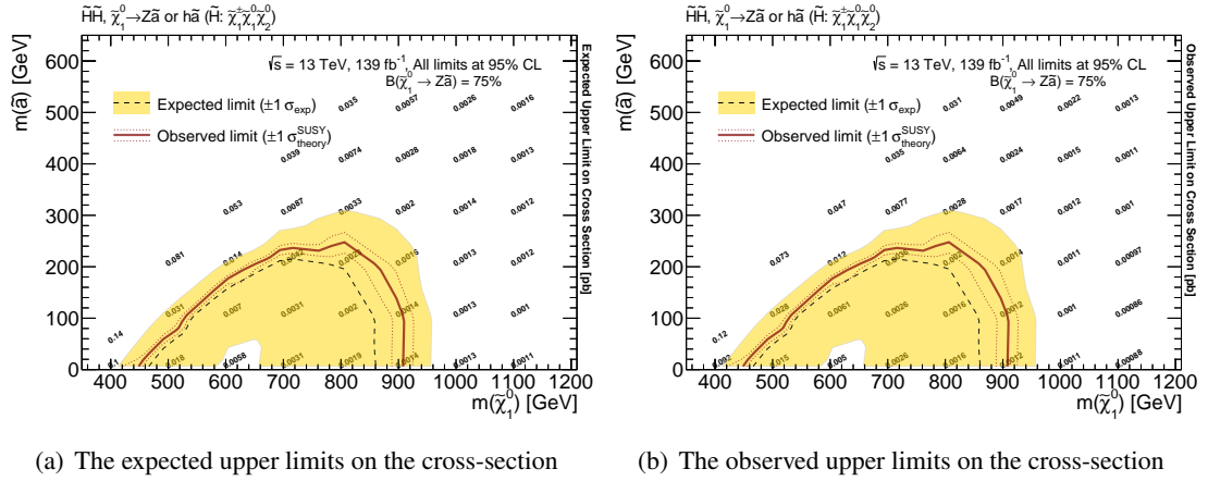
Figure S.42: Expected (a) and observed (b) upper limits on the cross-section with exclusion limits of the (\tilde{H}, \tilde{a}) model assuming \mathcal{B}(\tilde{\chi}_1^0 \rightarrow Z\tilde{a}) = 75\%
