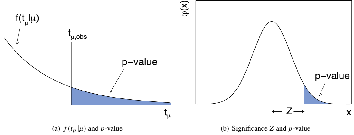
Figure 10.5: (a) Illustration of the relation between the p -value obtained from an observed value of the test statistic t_\mu , instead of s in Equation 10.4. (b) The standard normal distribution \varphi(x) = (1/\sqrt{2\pi})\exp(-x^2/2) showing the relation between the significance Z and the p -value [154].
