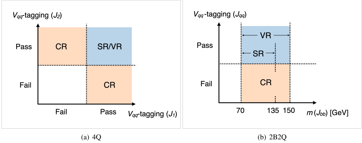
Figure 8.5: Schematics illustrating the relation between the SRs (VRs) and CRs in the (a) 4Q and (b) 2B2Q categories [49]. SRs (VRs) are required to pass boson tagging requirements for both two leading large- R jets, and the CRs are constructed by inverting the W_{qq}/Z_{qq} -tagging requirement for one of them. In the 2B2Q category, the J_{bb} mass window cuts in the CRs and VRs are loosened to increase data statistics and suppress signal contaminations.
