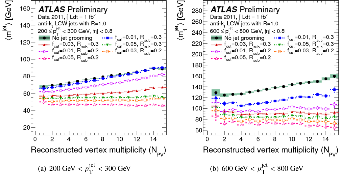
Figure 5.1: Performance of the jet grooming [107]. The distribution of mean uncalibrated jet mass with a function of the reconstructed vertex multiplicity ( N_{\text{PV}} ) in t\bar{t} MC sample is shown. The black line represents the mean mass of large- R jets without trimming. The red line represents the default ATLAS option for the trimming parameters.
