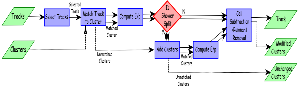
Figure D.1: A flowchart of the particle flow algorithm. The energy and momentum of clusters and tracks are modified by combining them [241].
