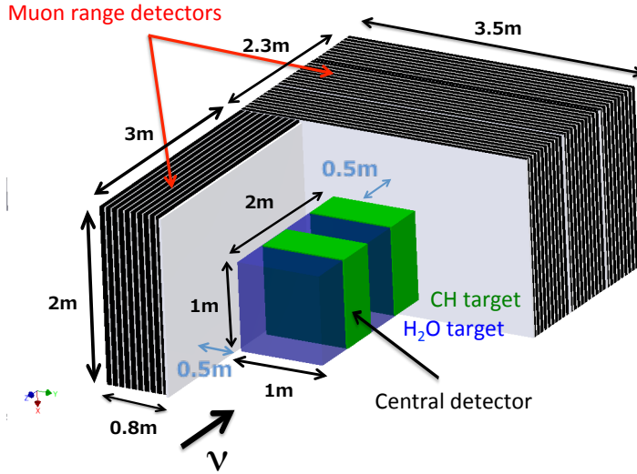
Figure 3: Schematic view of entire sets of detectors.
